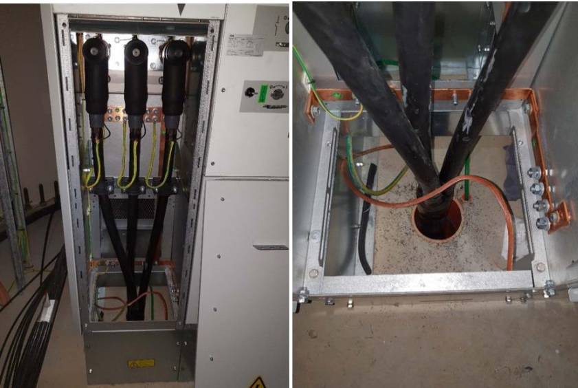
Cable terminations inside WTG in progress
